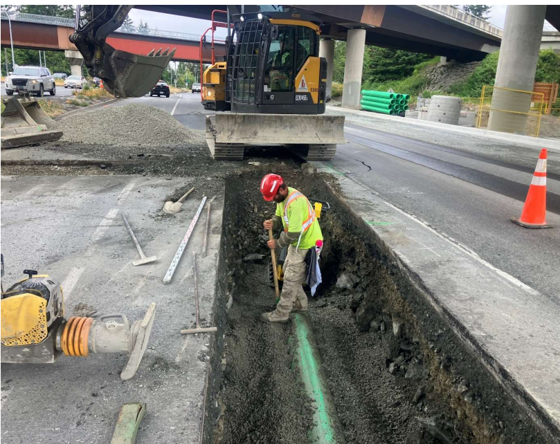
Drainage works along Burnside Road West, near Island Highway intersection
